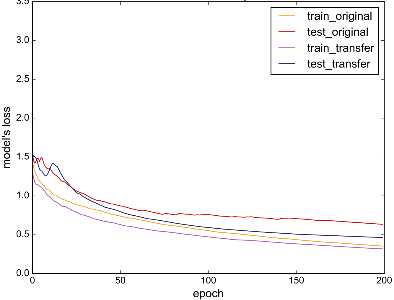
Source: InlineSkate - Target: FaceFour
