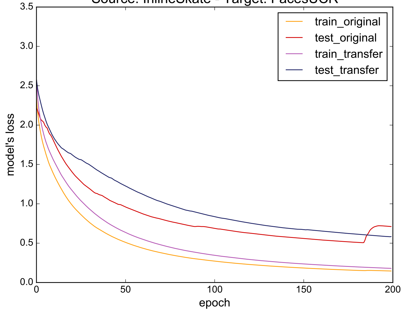
Source: InlineSkate - Target: FacesUCR
