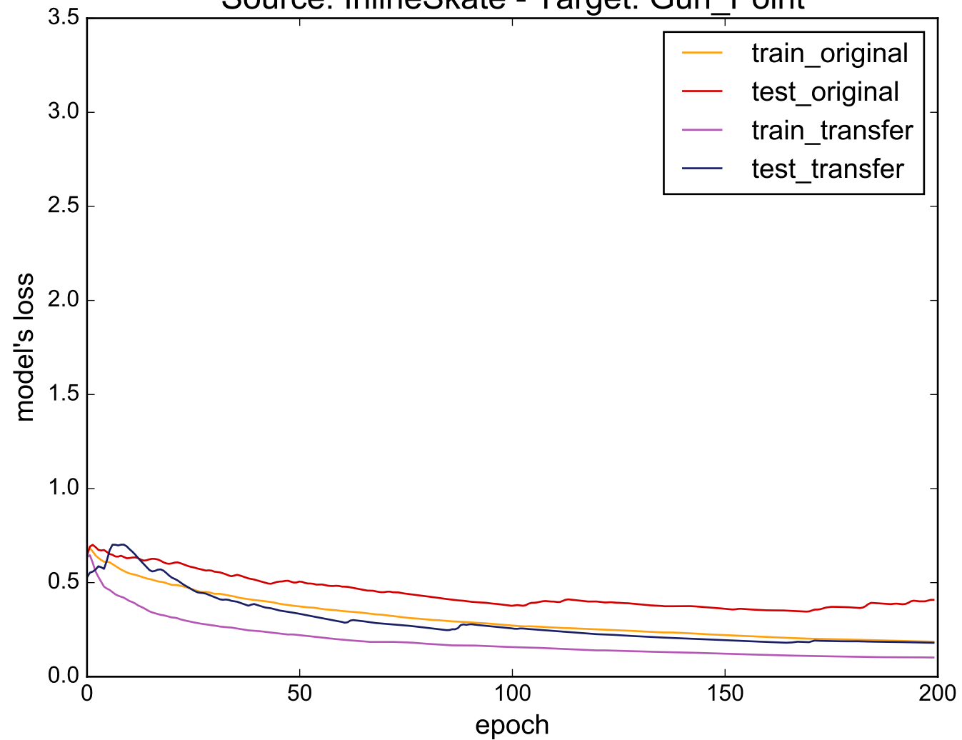
Source: InlineSkate - Target: Gun_Point
