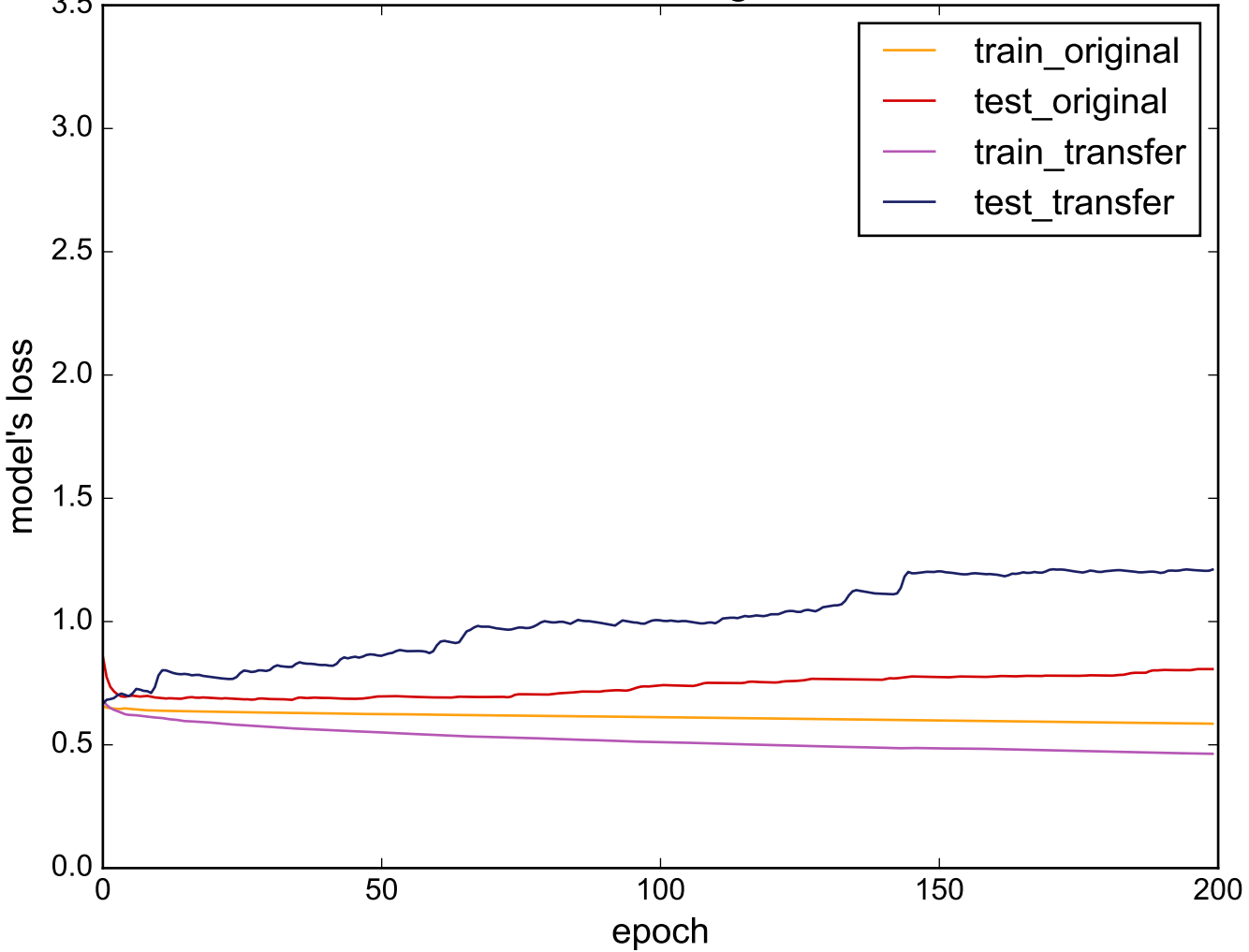
Source: InlineSkate - Target: HandOutlines
