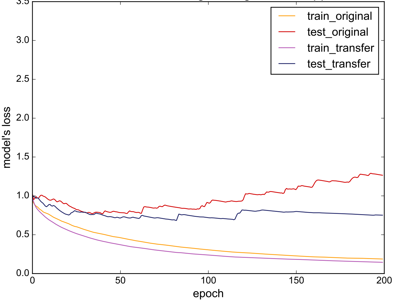
Source: InlineSkate - Target: LargeKitchenAppliances
