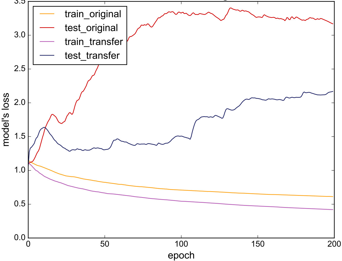
Source: InlineSkate - Target: Meat
