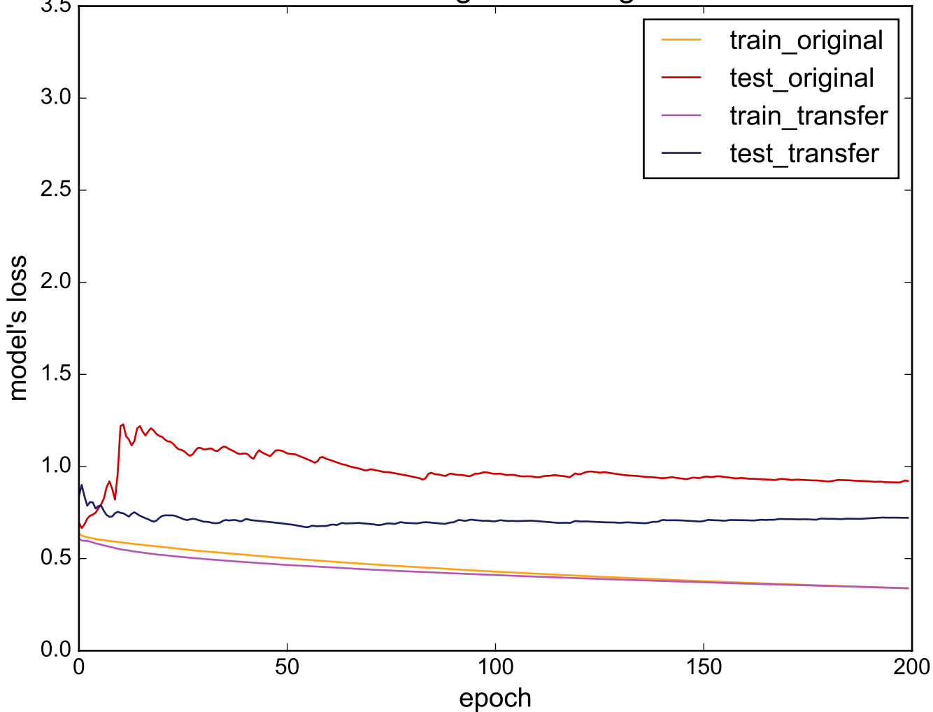
Source: InlineSkate - Target: PhalangesOutlinesCorrect
