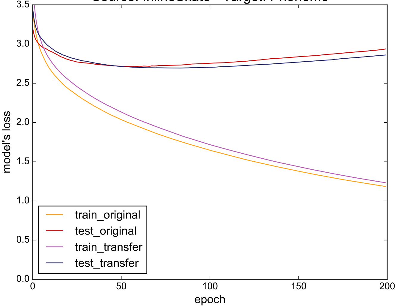
Source: InlineSkate - Target: Phoneme
