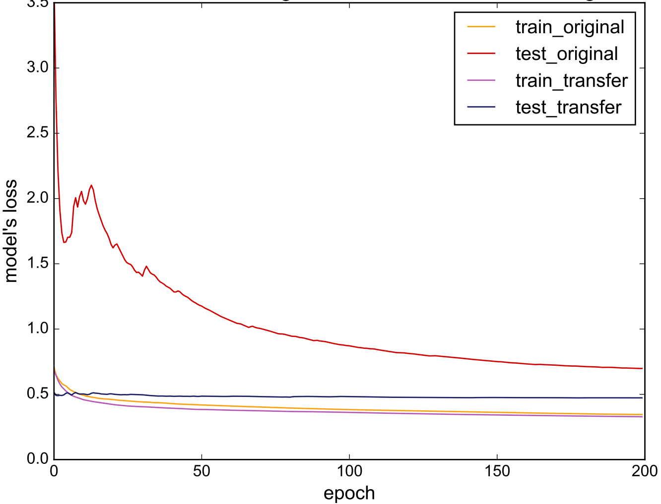
Source: InlineSkate - Target: ProximalPhalanxOutlineAgeGroup
