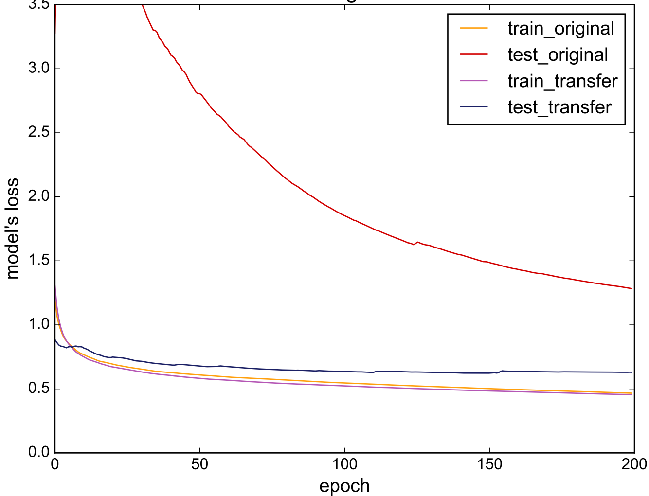
Source: InlineSkate - Target: ProximalPhalanxTW
