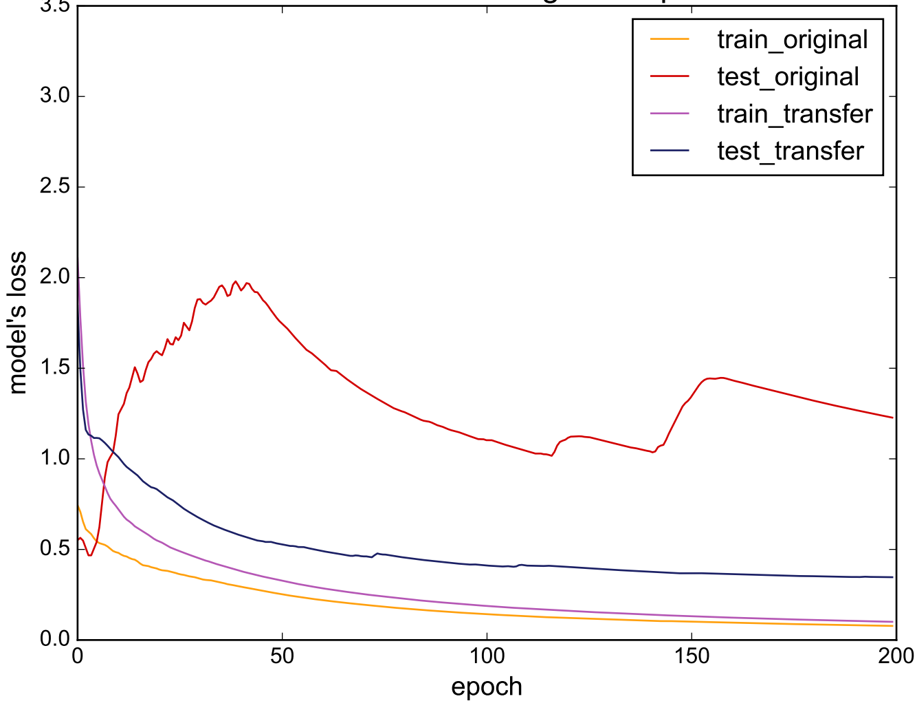
Source: InlineSkate - Target: ShapeletSim
