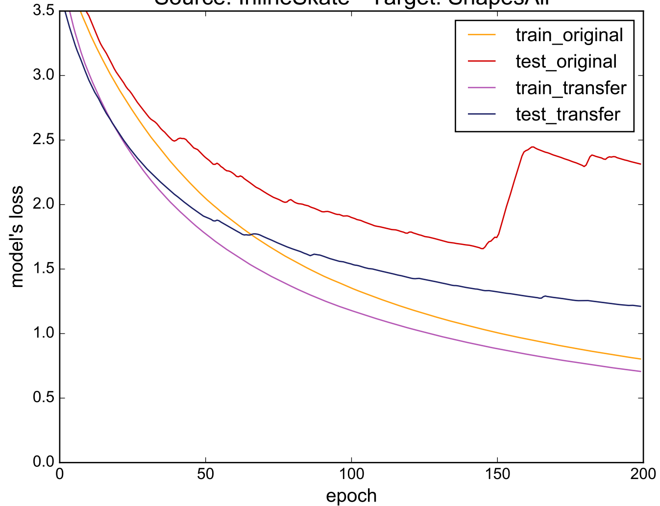
Source: InlineSkate - Target: ShapesAll
