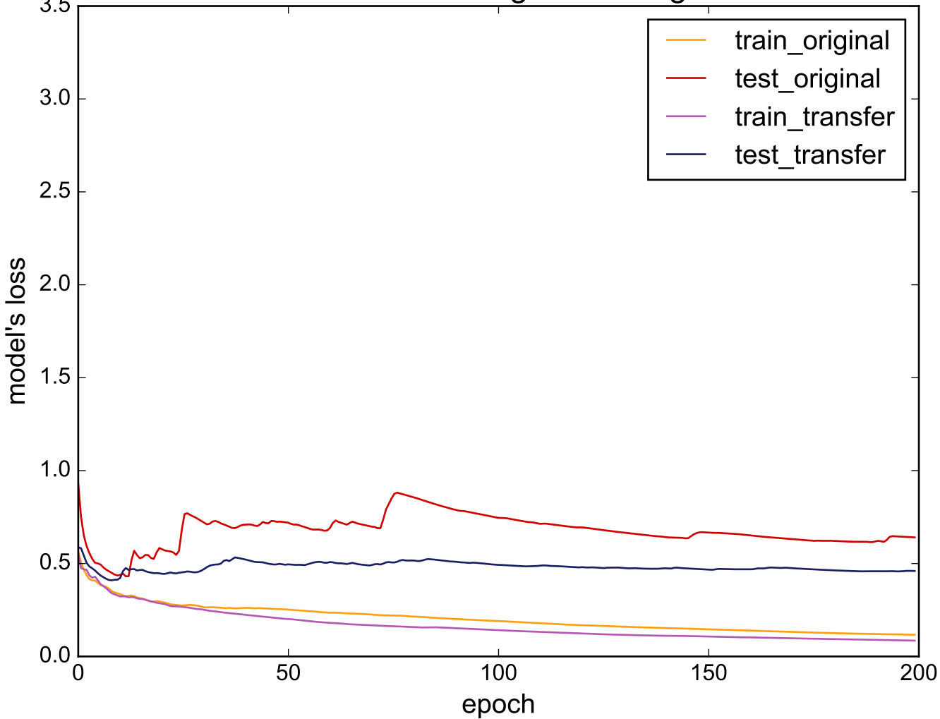
Source: InlineSkate - Target: ToeSegmentation2
