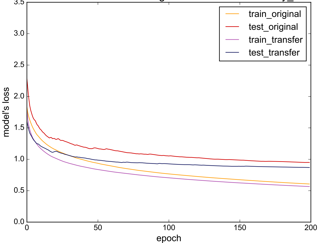
Source: InlineSkate - Target: uWaveGestureLibrary_X
