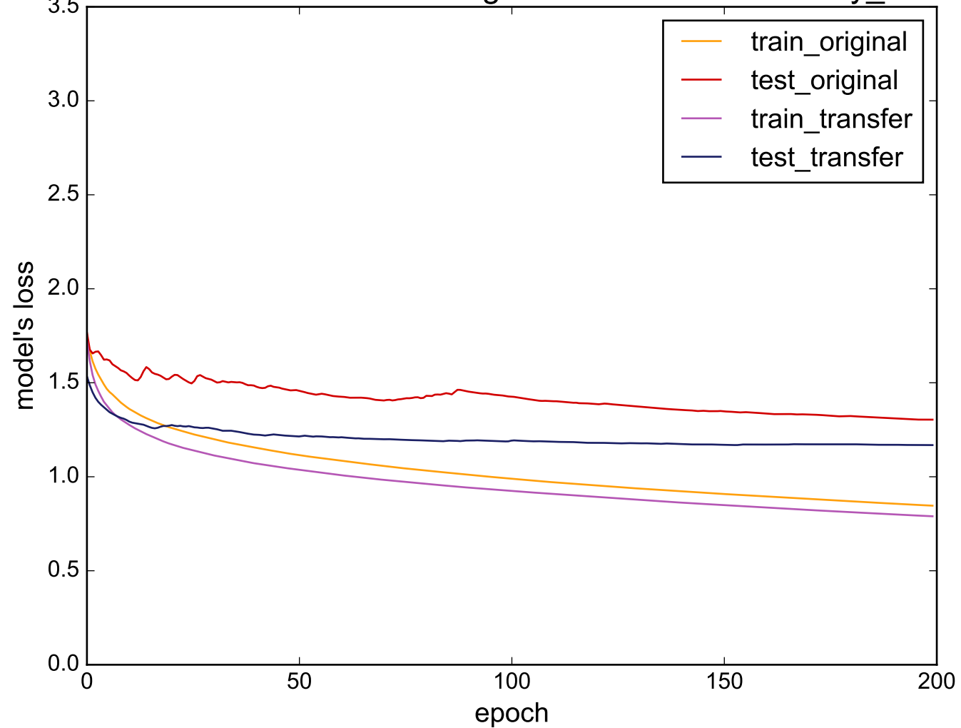
Source: InlineSkate - Target: uWaveGestureLibrary_Y
