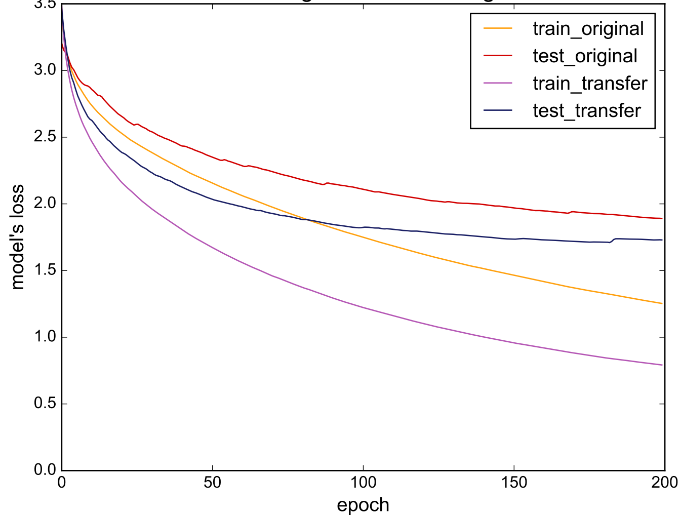
Source: InsectWingbeatSound - Target: 50words
