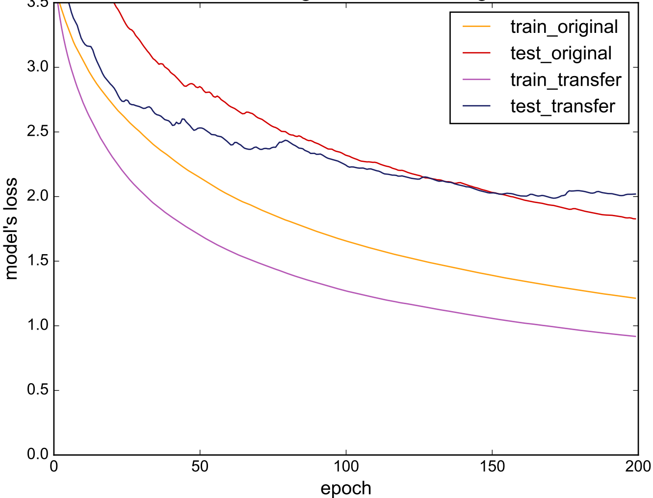
Source: InsectWingbeatSound - Target: Adiac
