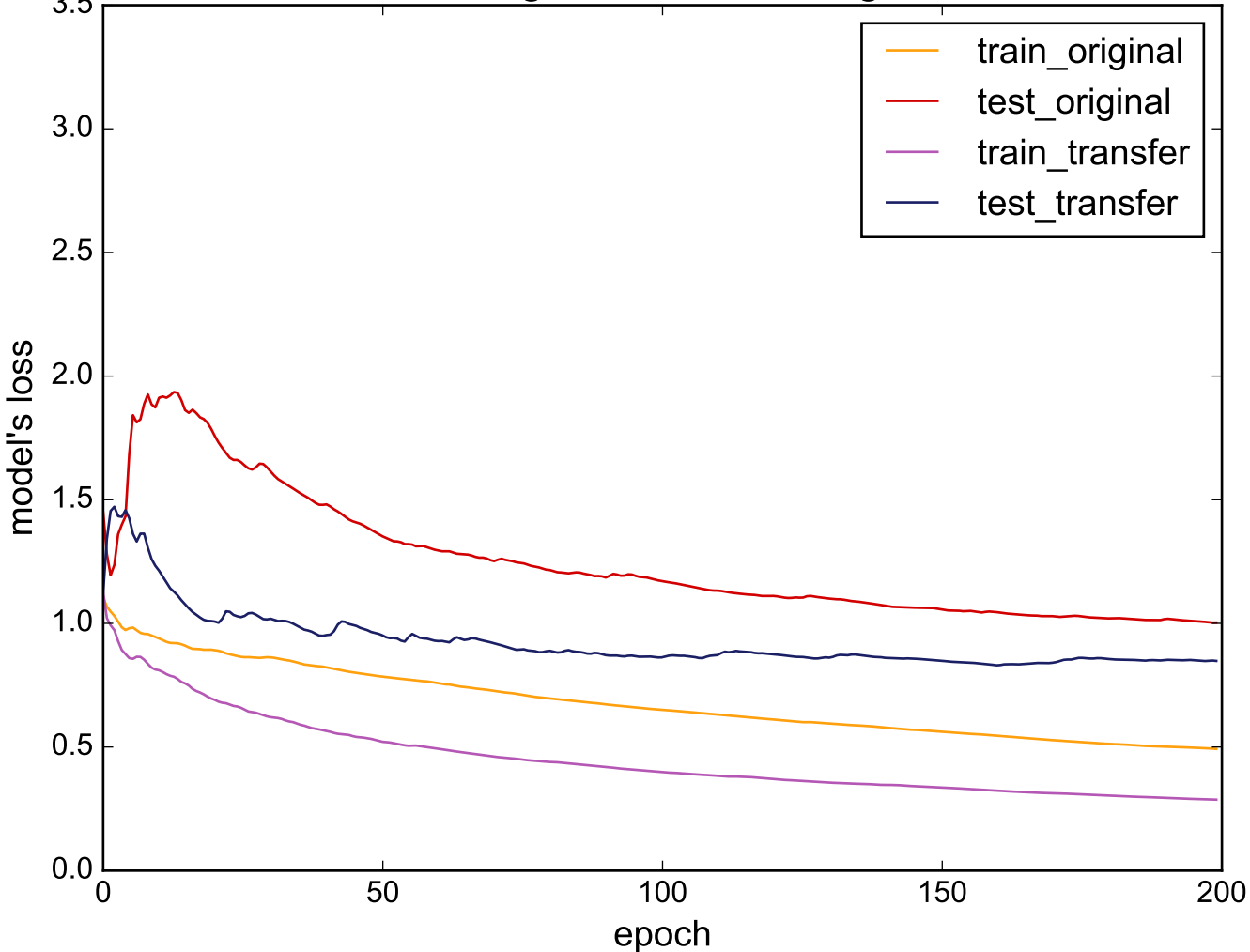
Source: InsectWingbeatSound - Target: ArrowHead
