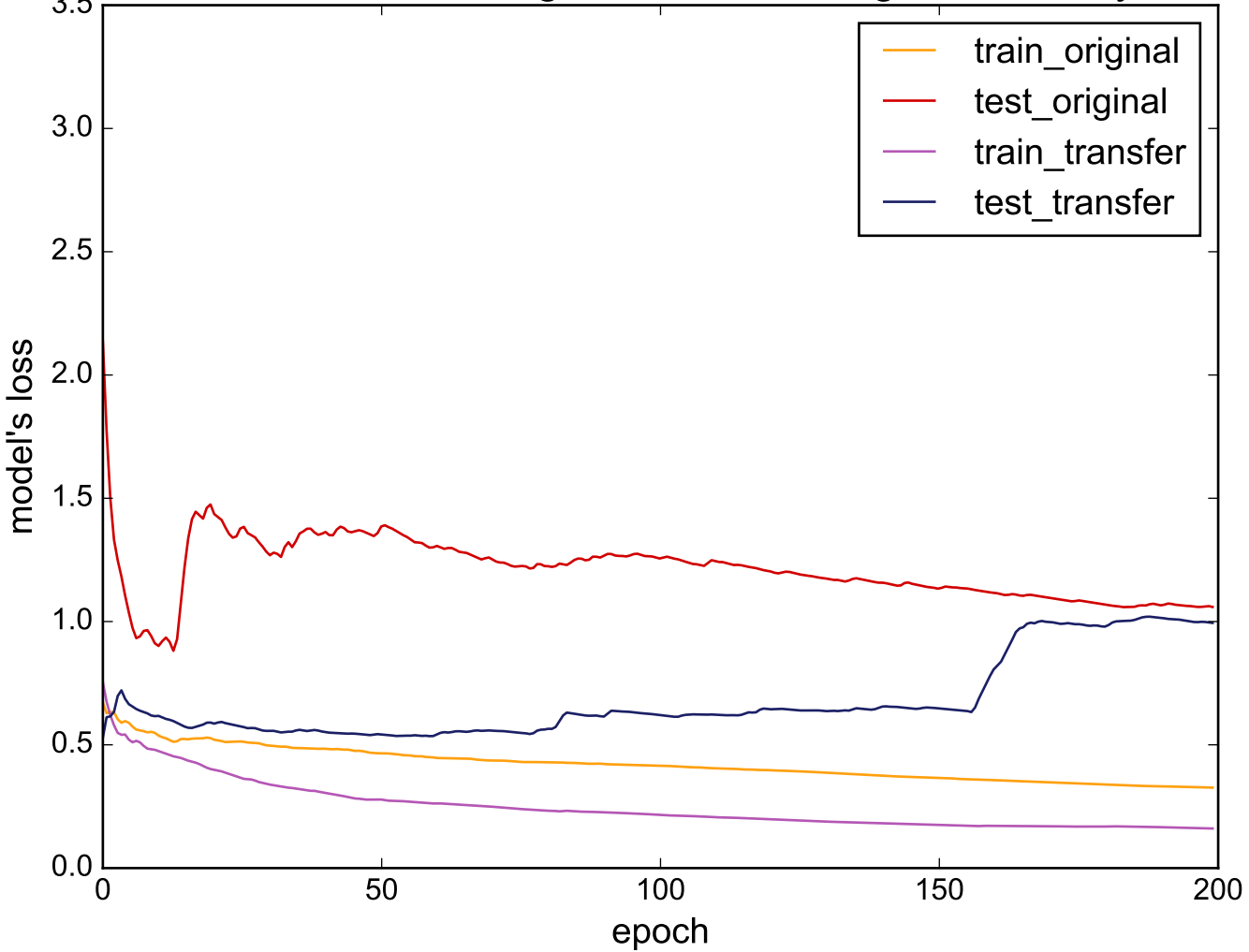
Source: InsectWingbeatSound - Target: BeetleFly
