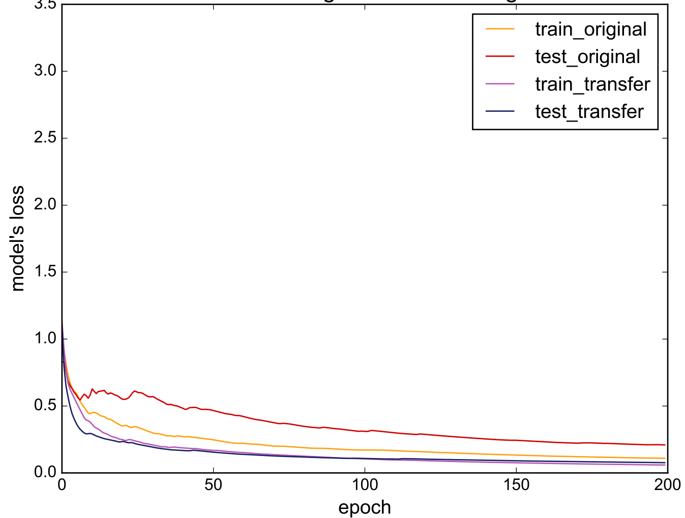
Source: InsectWingbeatSound - Target: CBF
