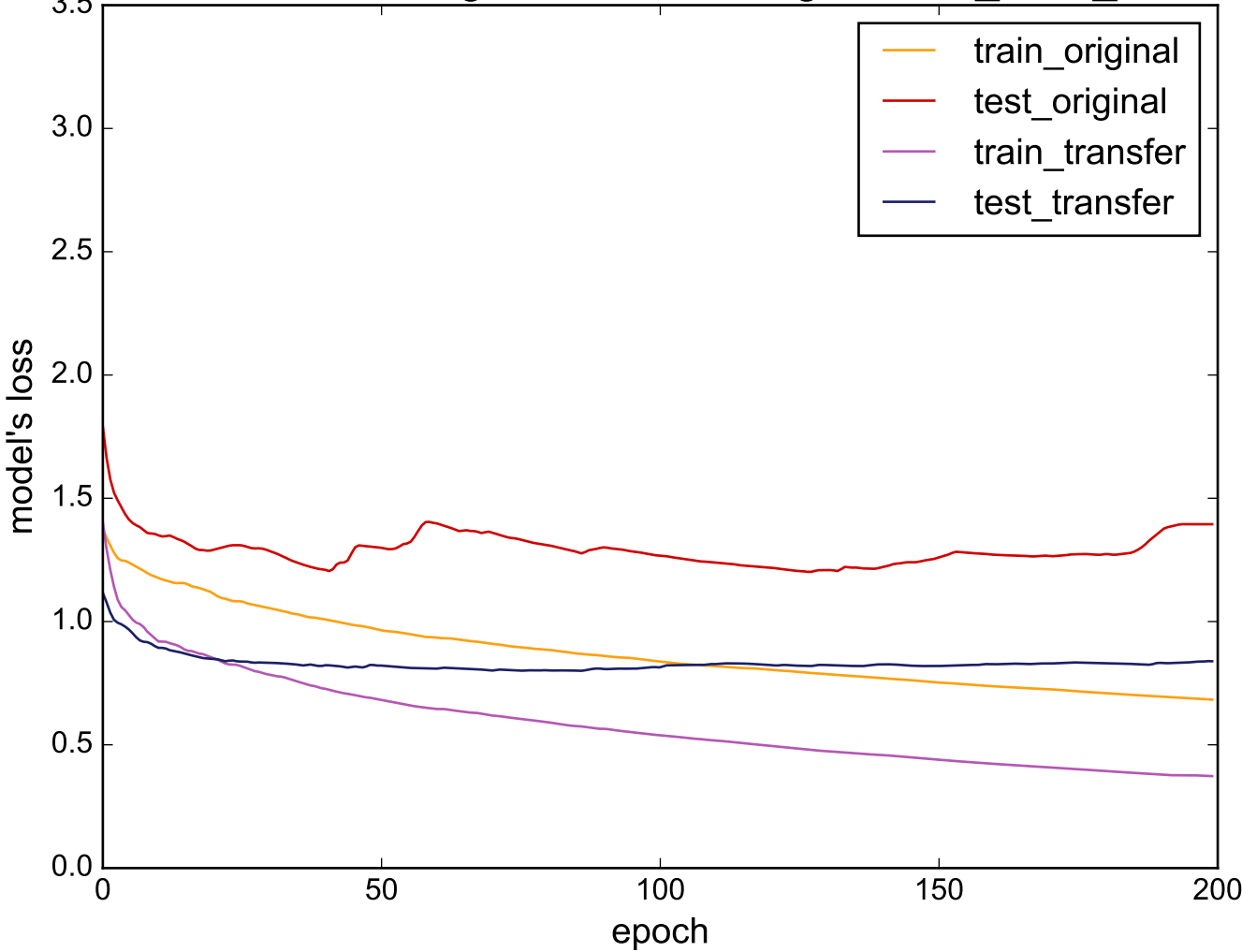
Source: InsectWingbeatSound - Target: CinC_ECG_torso
