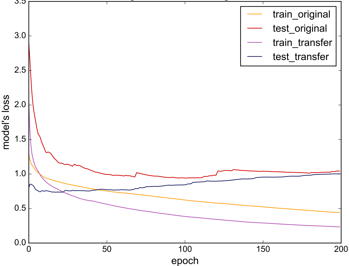
Source: InsectWingbeatSound - Target: DistalPhalanxTW
