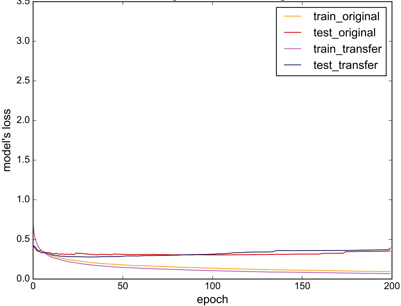
Source: InsectWingbeatSound - Target: ECG5000
