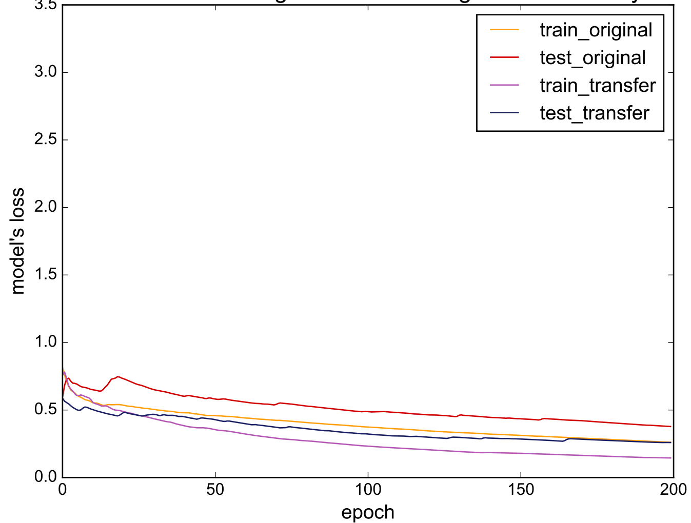
Source: InsectWingbeatSound - Target: ECGFiveDays
