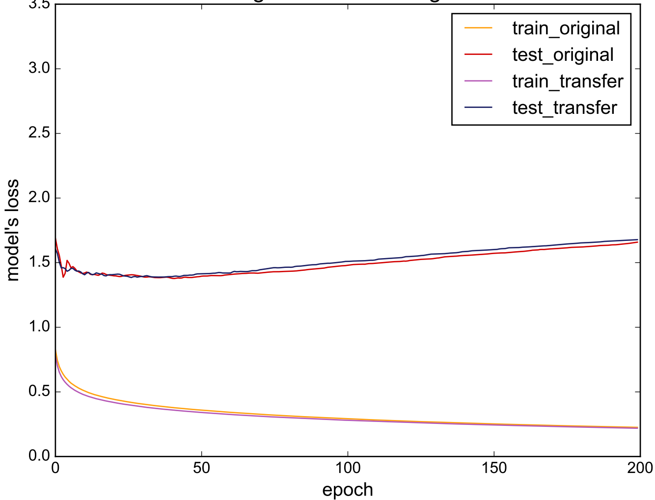
Source: InsectWingbeatSound - Target: ElectricDevices
