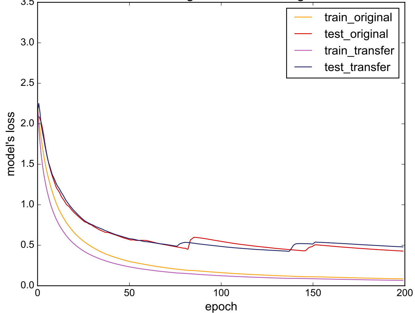
Source: InsectWingbeatSound - Target: FaceAll
