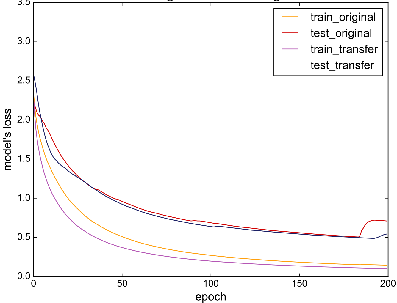
Source: InsectWingbeatSound - Target: FacesUCR
