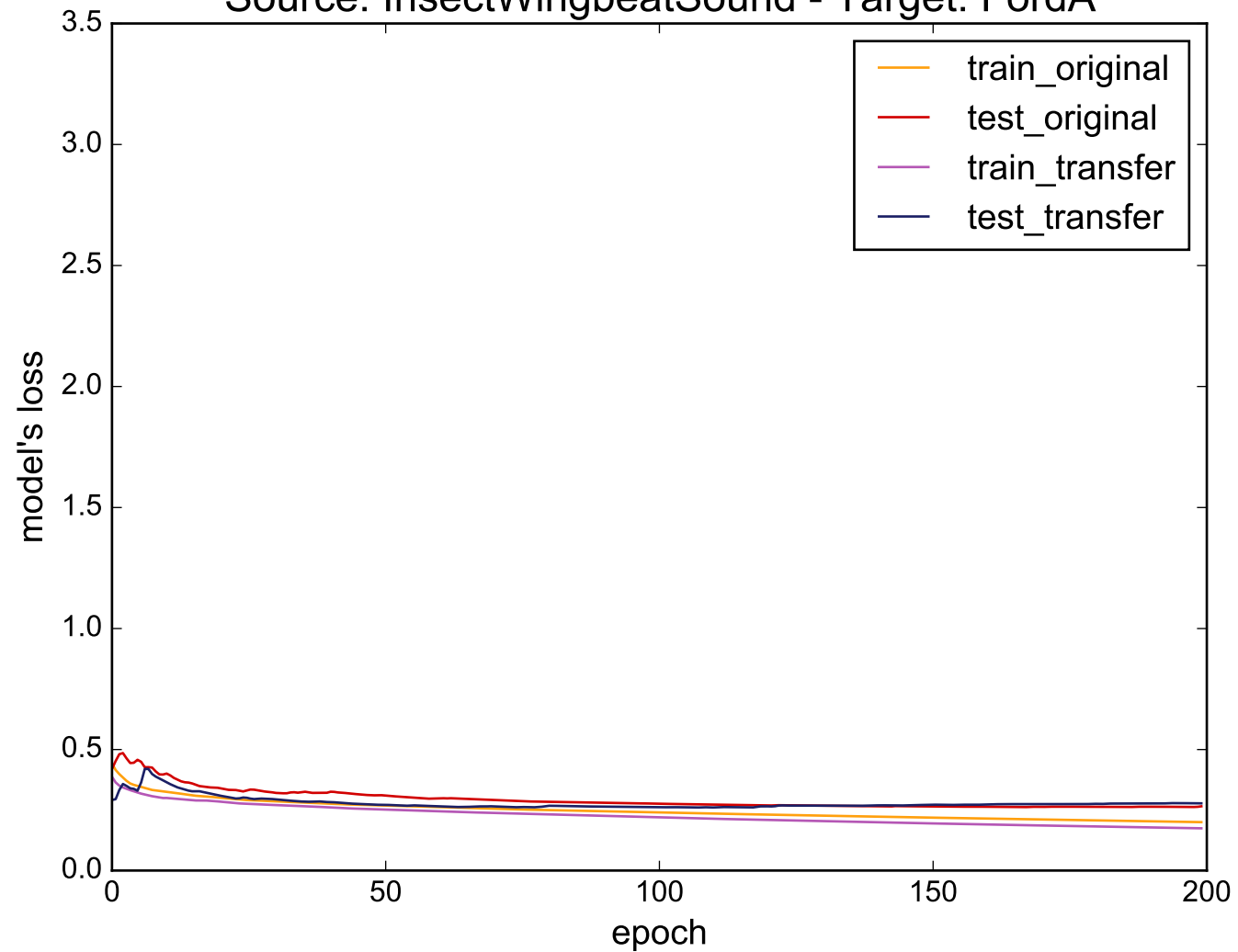
Source: InsectWingbeatSound - Target: FordA
