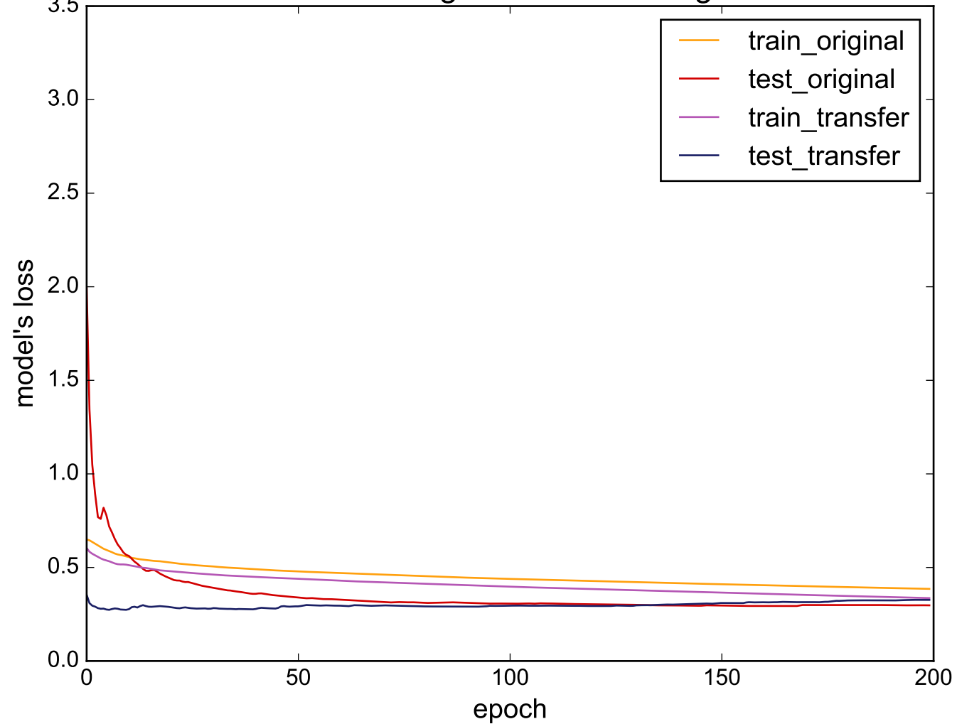
Source: InsectWingbeatSound - Target: FordB
