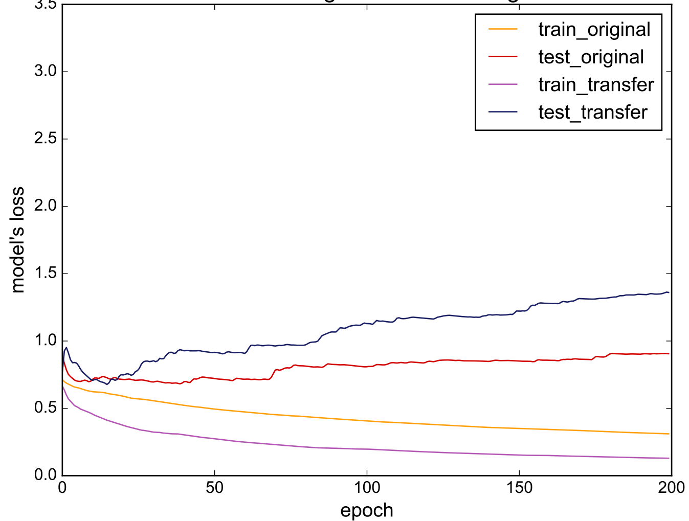
Source: InsectWingbeatSound - Target: Ham
