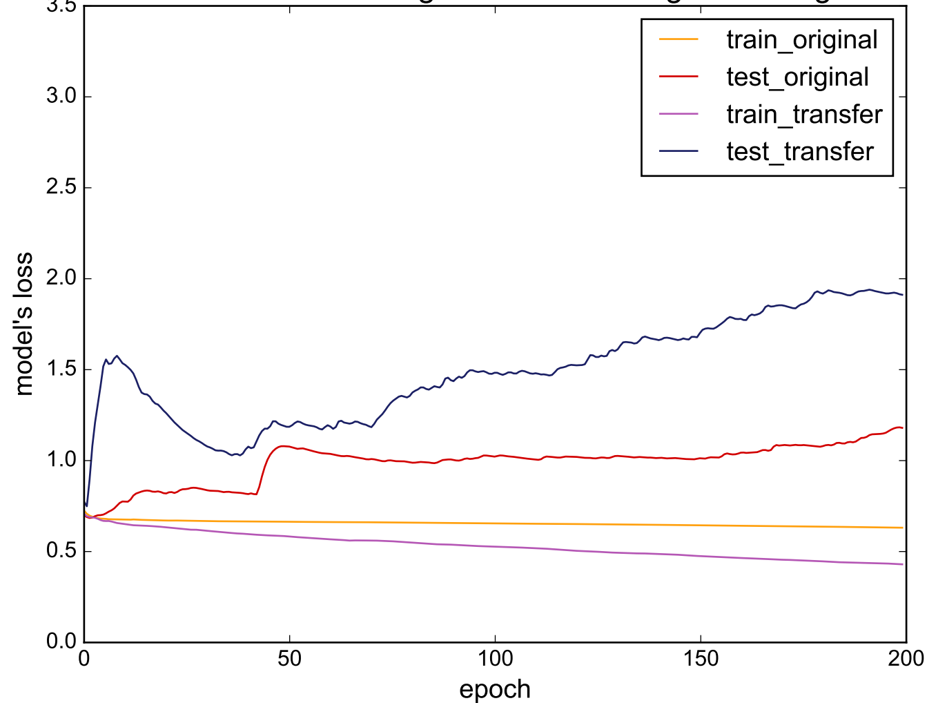
Source: InsectWingbeatSound - Target: Herring
