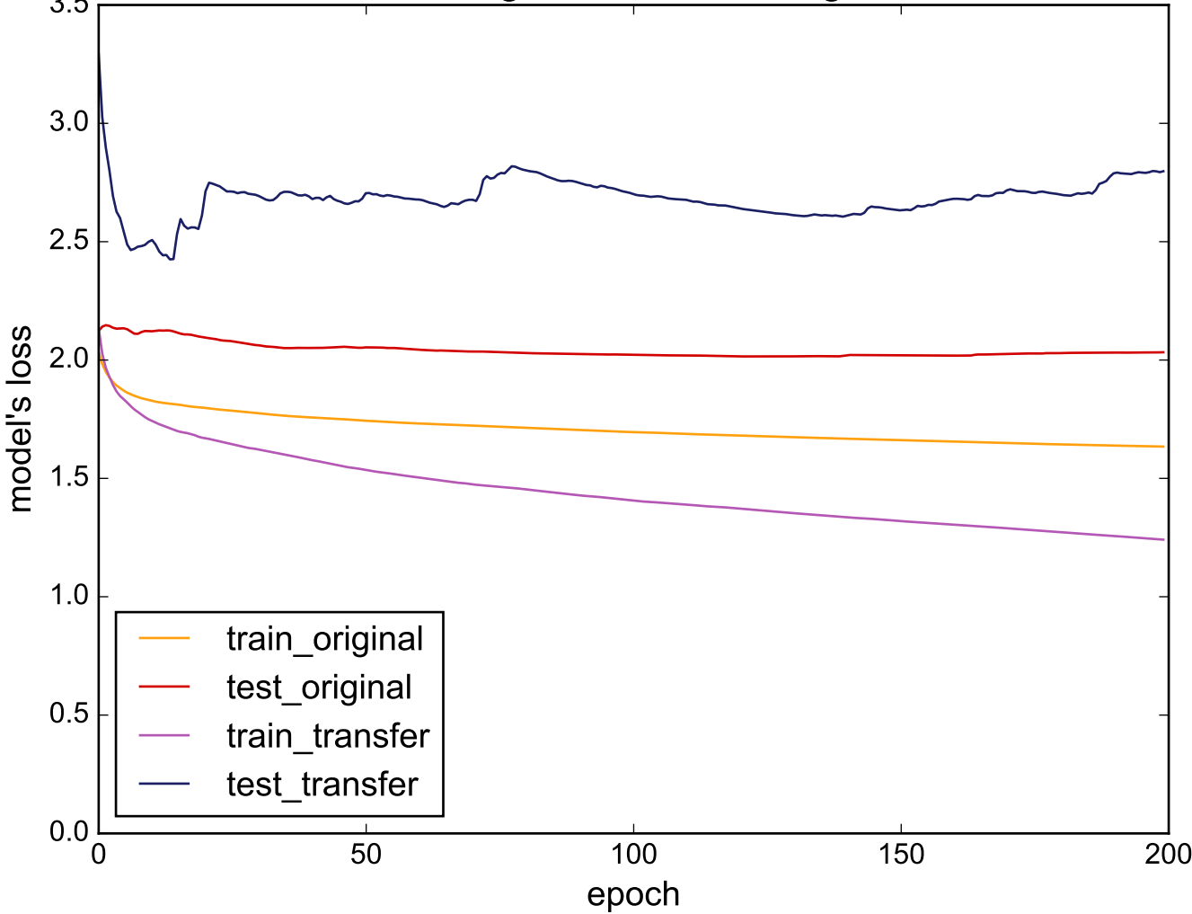
Source: InsectWingbeatSound - Target: InlineSkate
