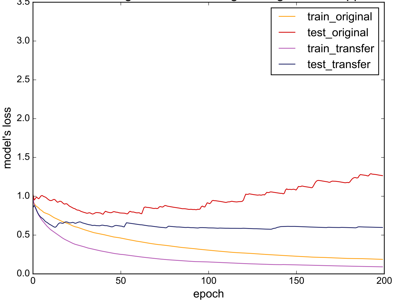
Source: InsectWingbeatSound - Target: LargeKitchenAppliances
