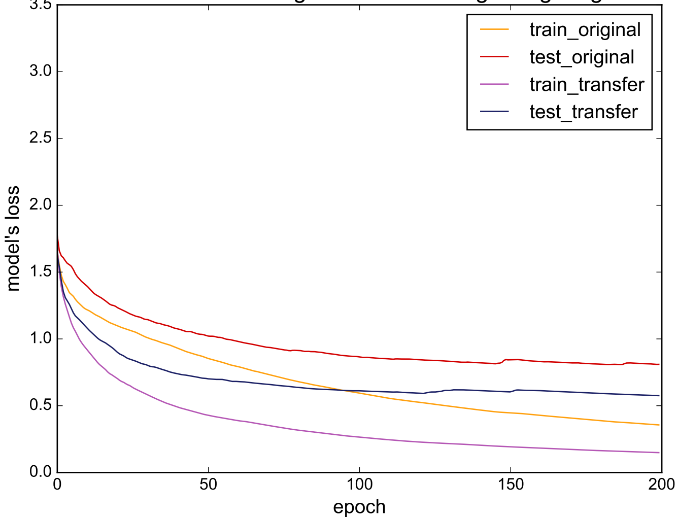
Source: InsectWingbeatSound - Target: Lighting7
