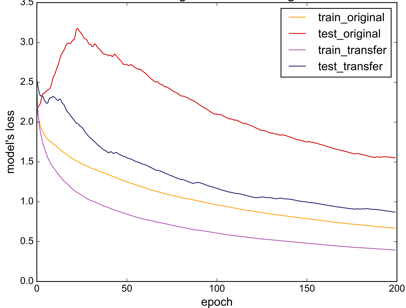
Source: InsectWingbeatSound - Target: MALLAT
