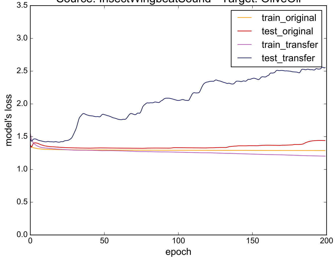
Source: InsectWingbeatSound - Target: OliveOil
