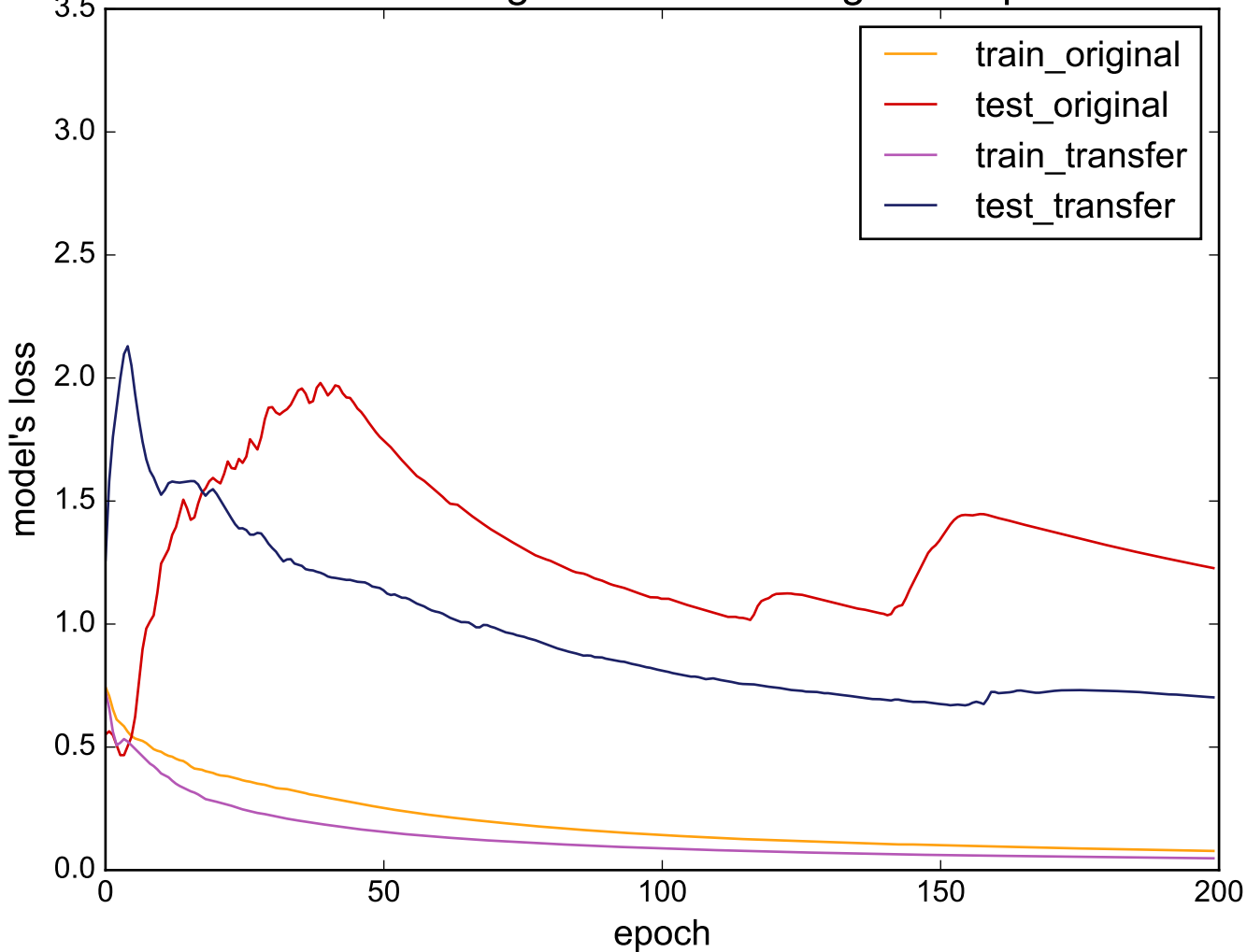
Source: InsectWingbeatSound - Target: ShapeletSim
