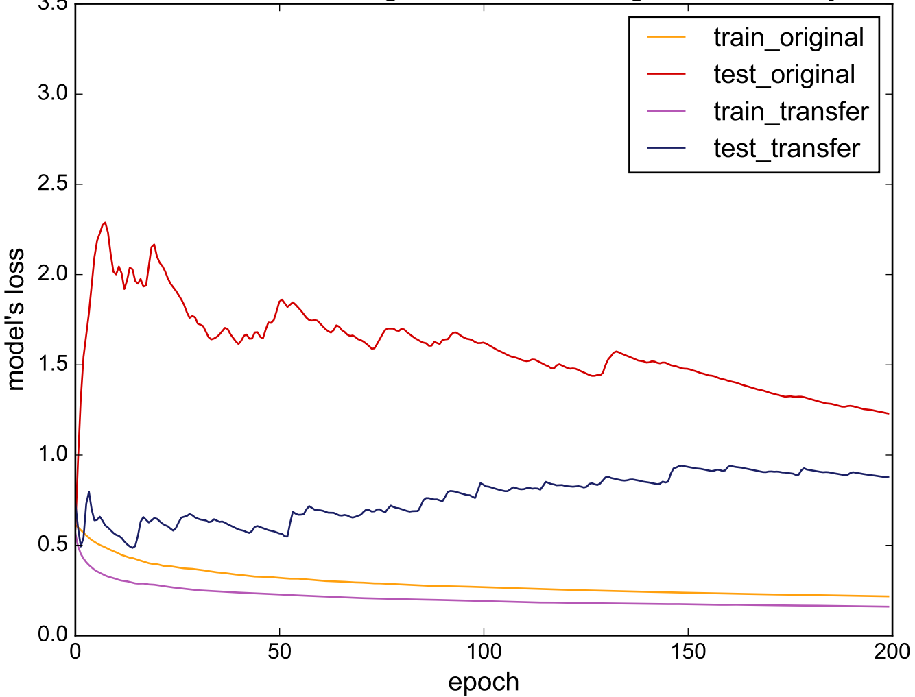
Source: InsectWingbeatSound - Target: Strawberry
