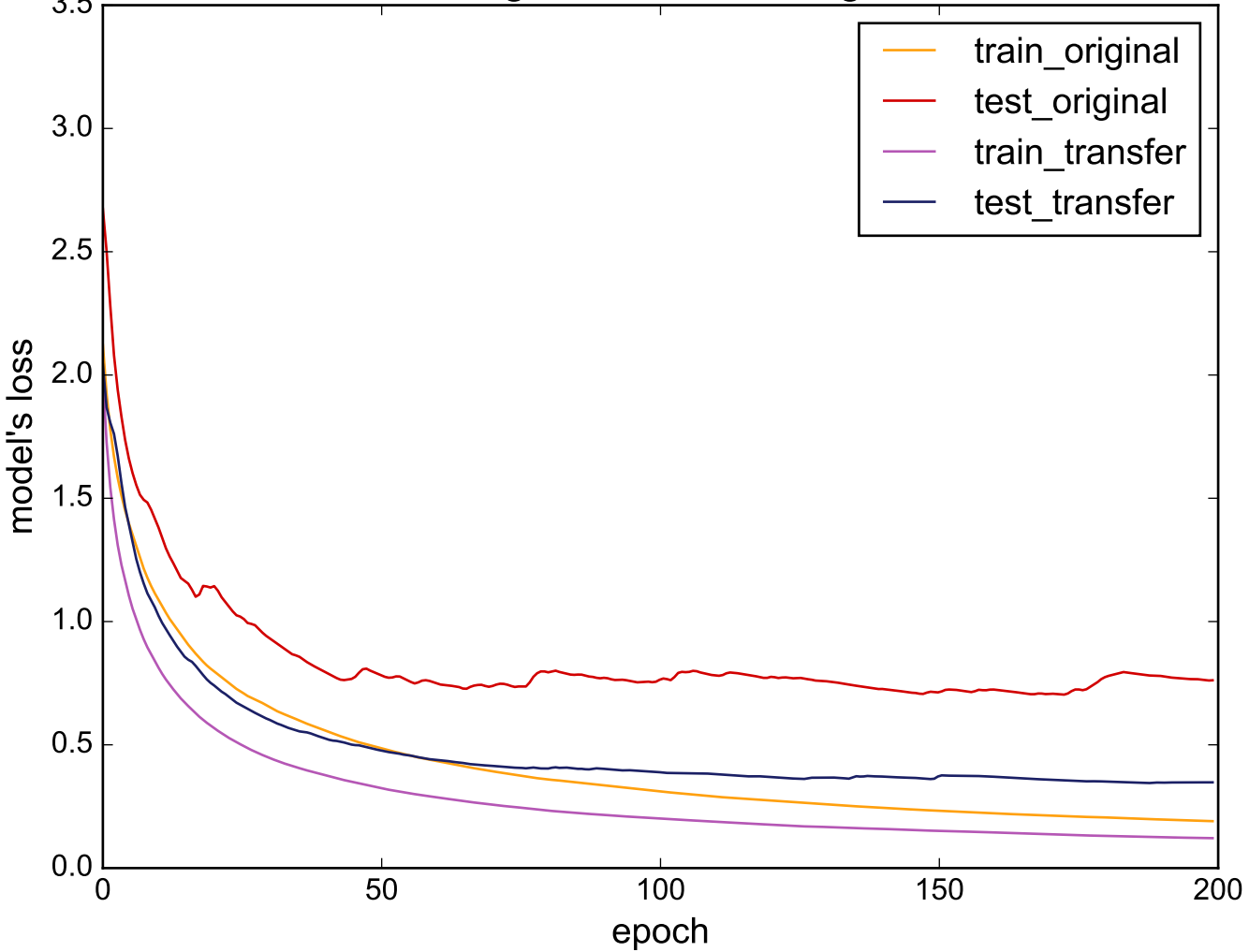
Source: InsectWingbeatSound - Target: SwedishLeaf
