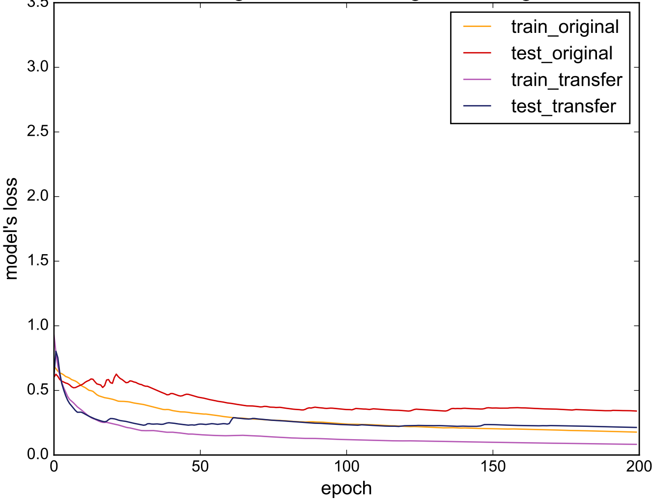
Source: InsectWingbeatSound - Target: ToeSegmentation1
