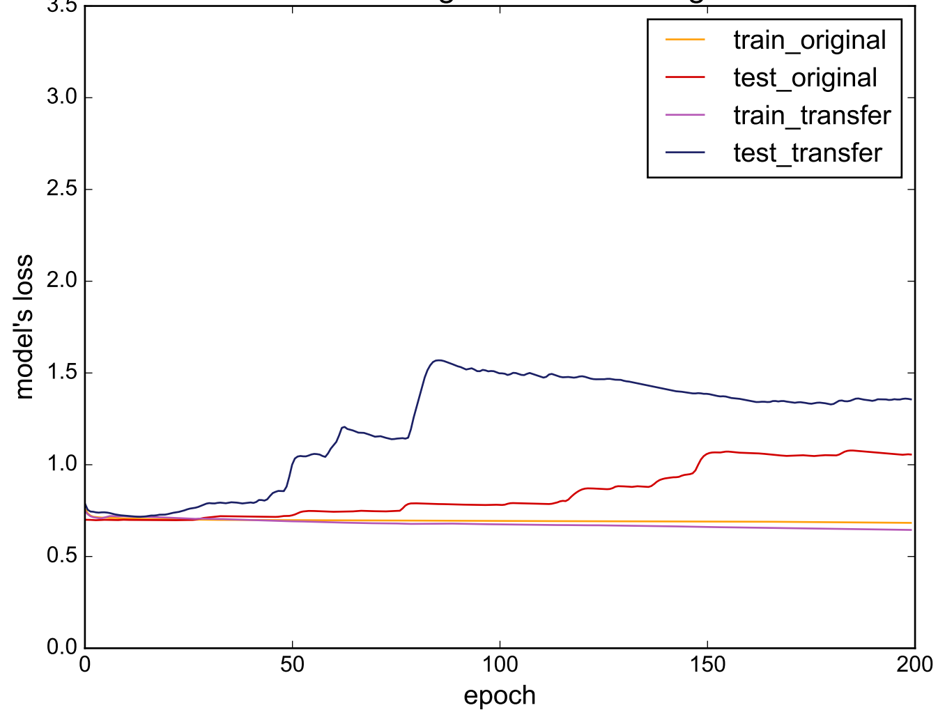
Source: InsectWingbeatSound - Target: Wine
