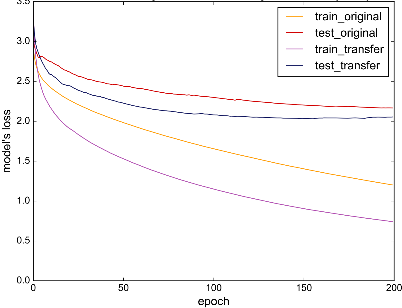
Source: InsectWingbeatSound - Target: WordsSynonyms
