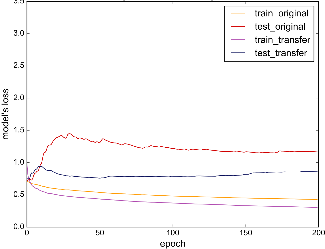
Source: InsectWingbeatSound - Target: WormsTwoClass
