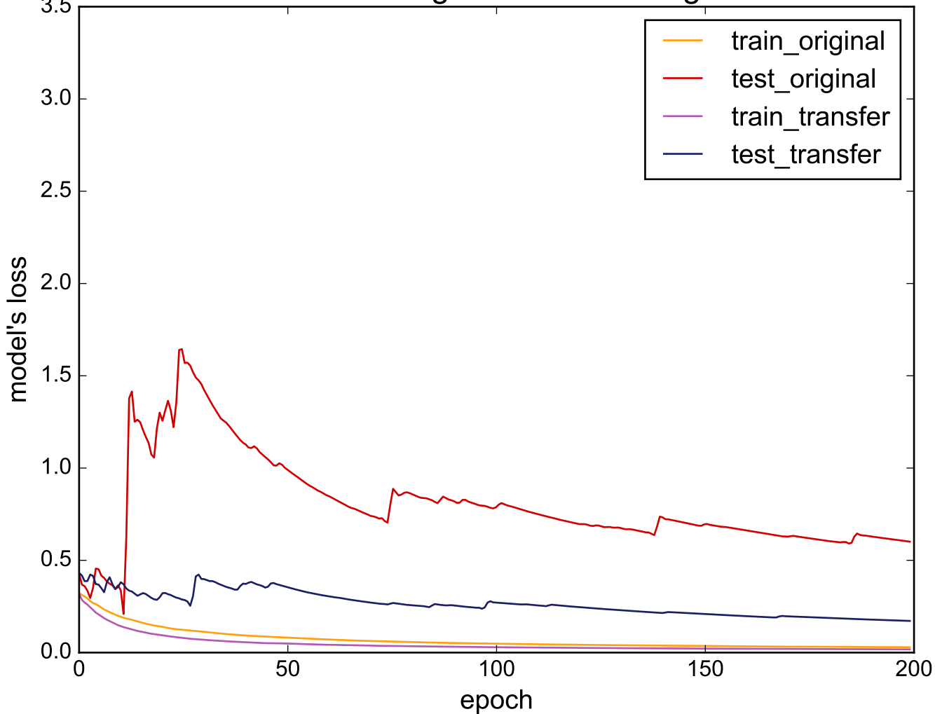
Source: InsectWingbeatSound - Target: wafer
