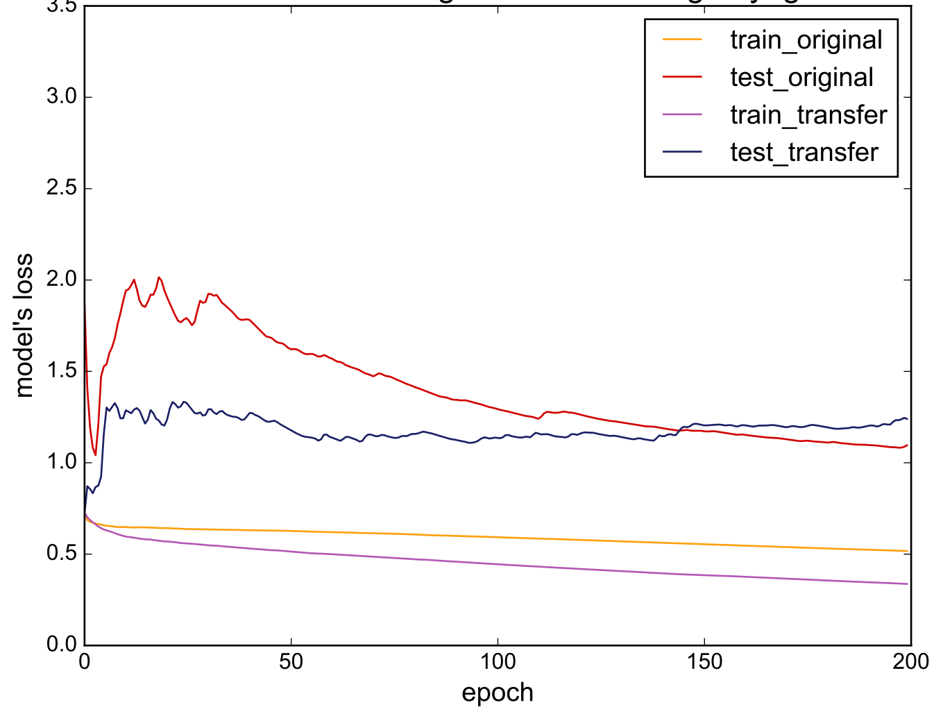
Source: InsectWingbeatSound - Target: yoga
