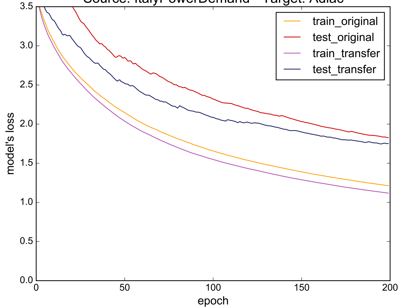
Source: ItalyPowerDemand - Target: Adiac
