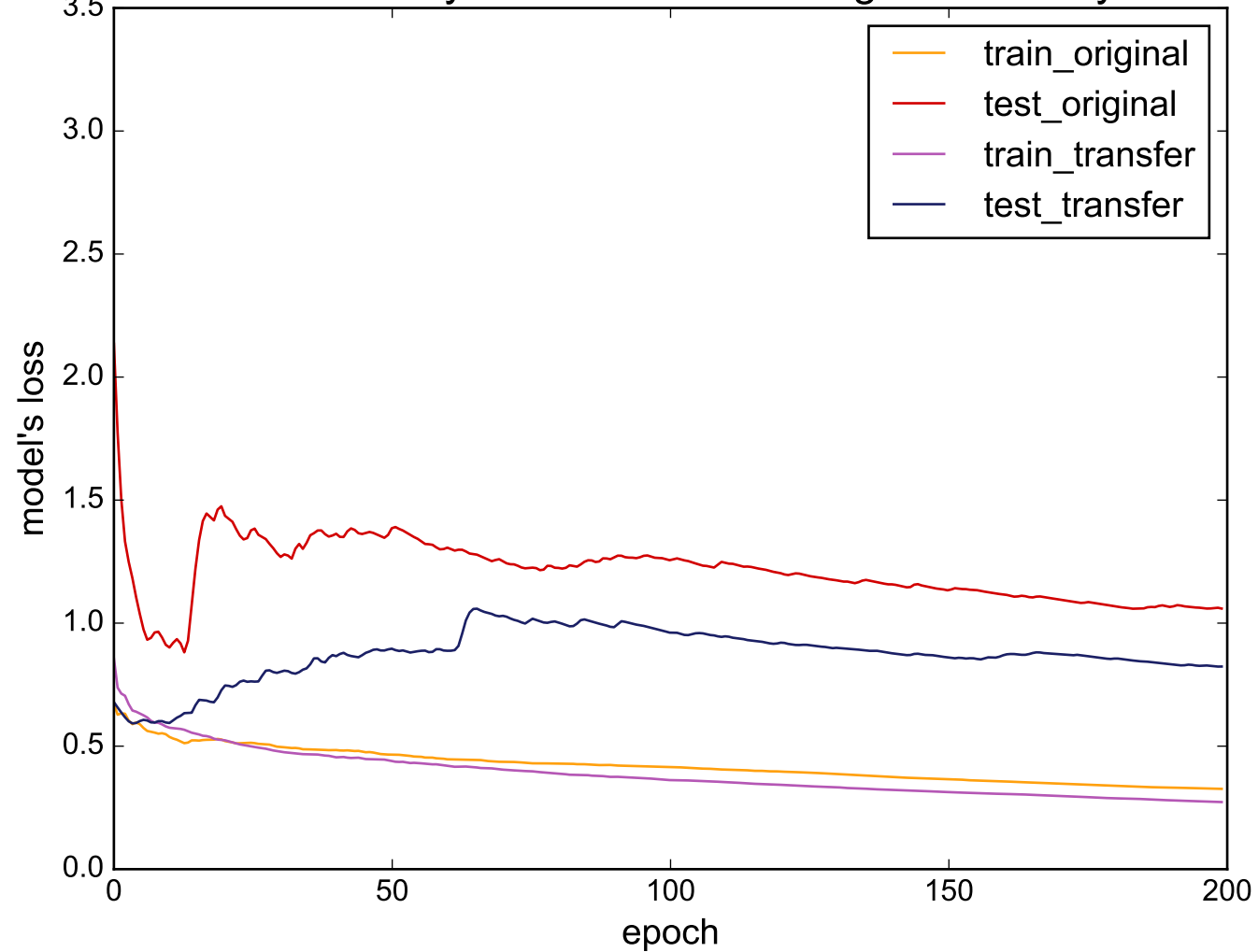
Source: ItalyPowerDemand - Target: BeetleFly
