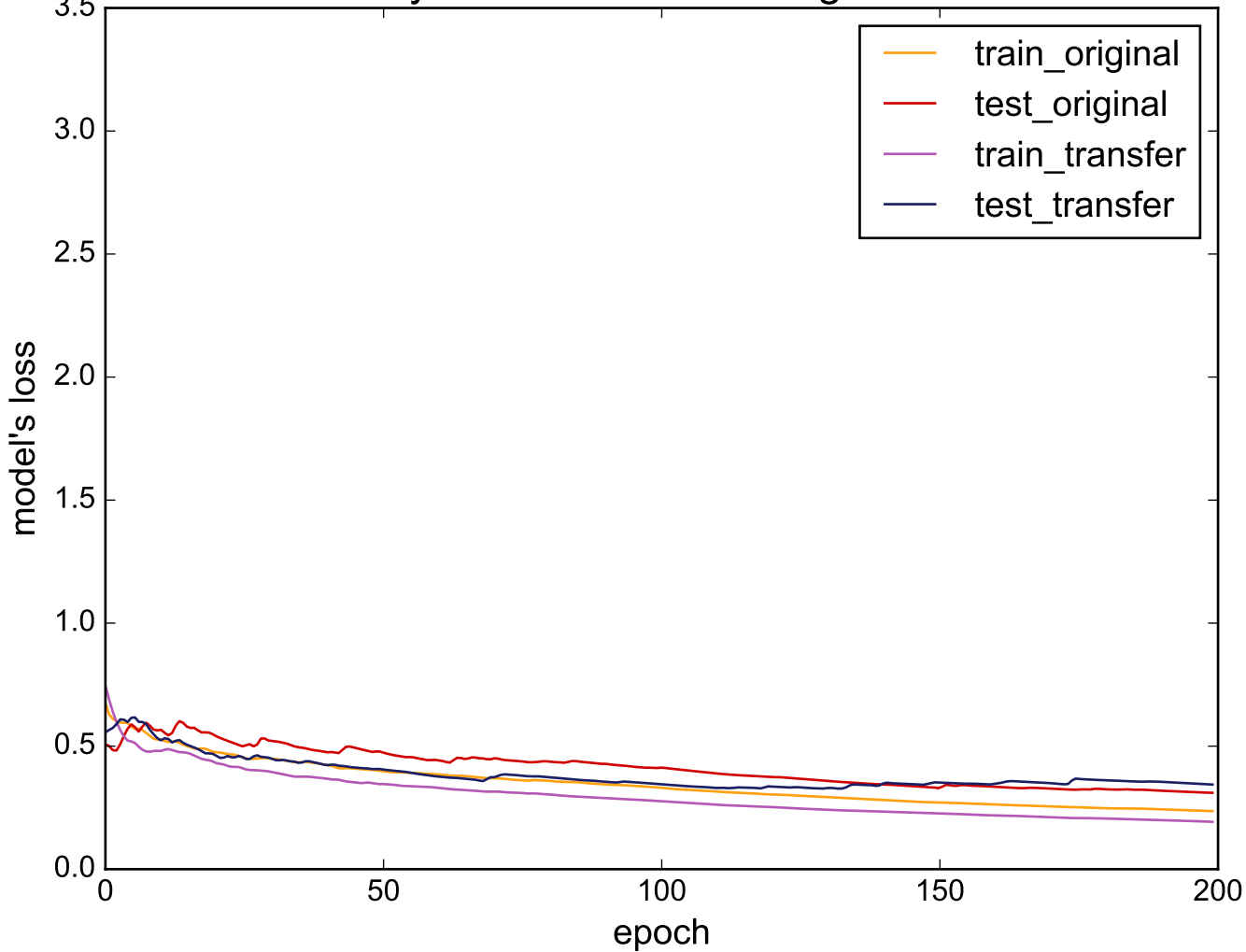
Source: ItalyPowerDemand - Target: BirdChicken
