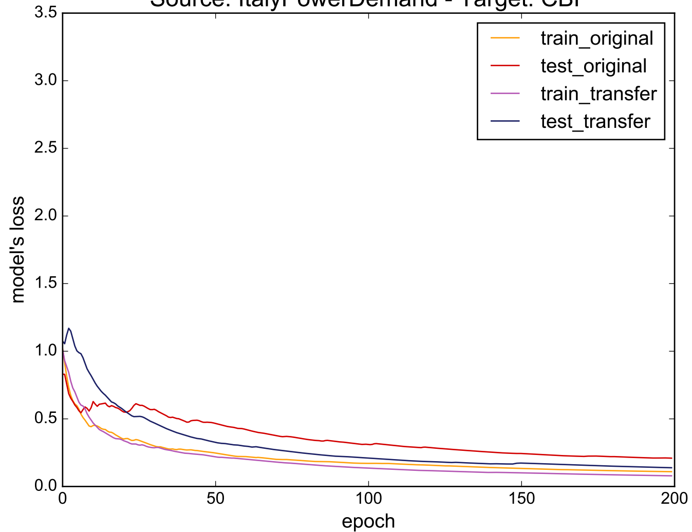
Source: ItalyPowerDemand - Target: CBF
