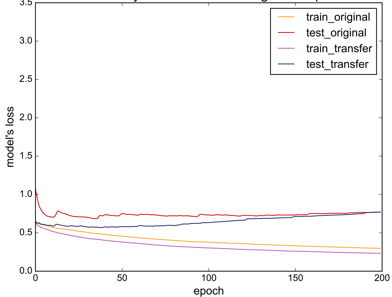
Source: ItalyPowerDemand - Target: Computers
